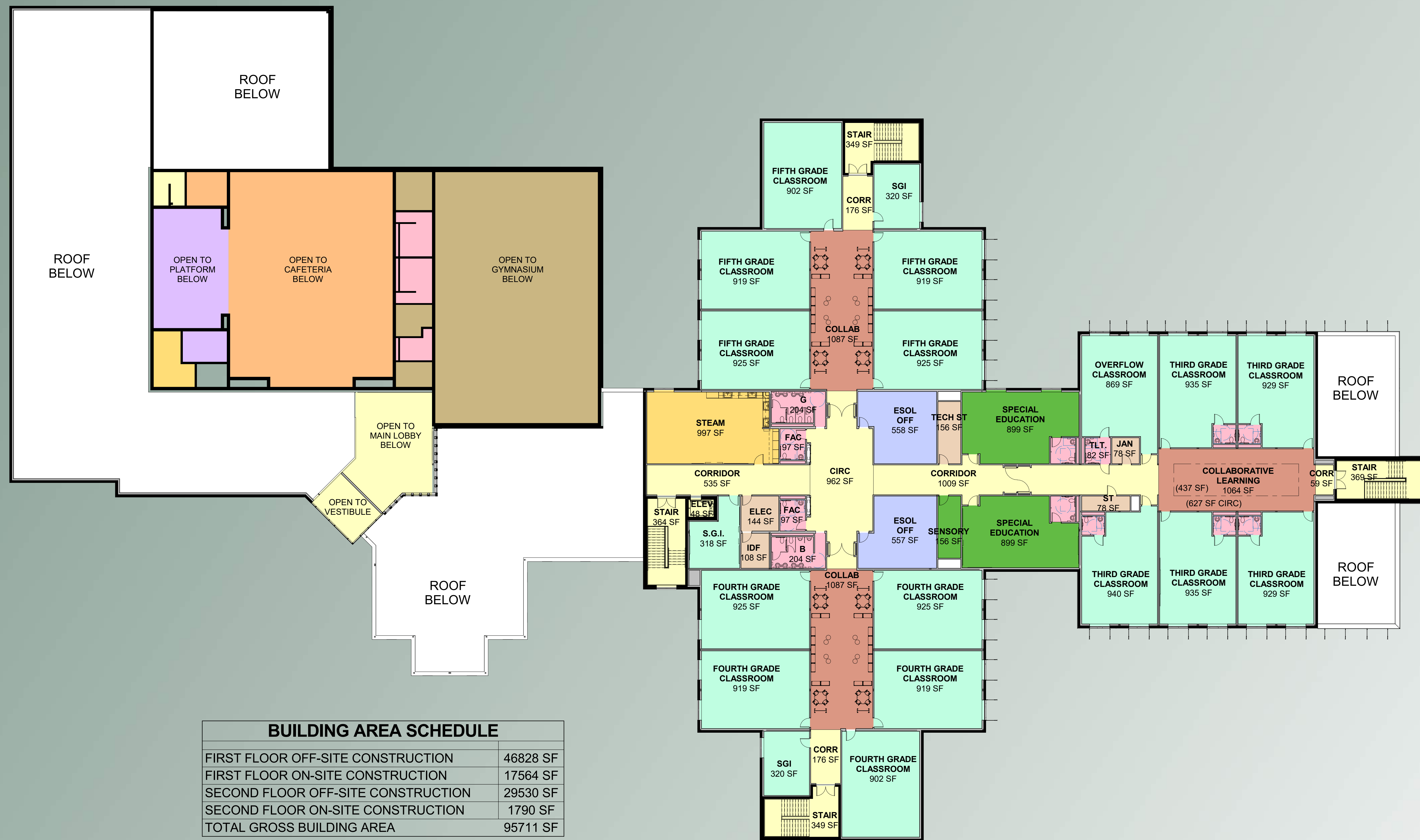
SECOND FLOOR PLAN - OPTION 5 1/16" = 1'-0"
